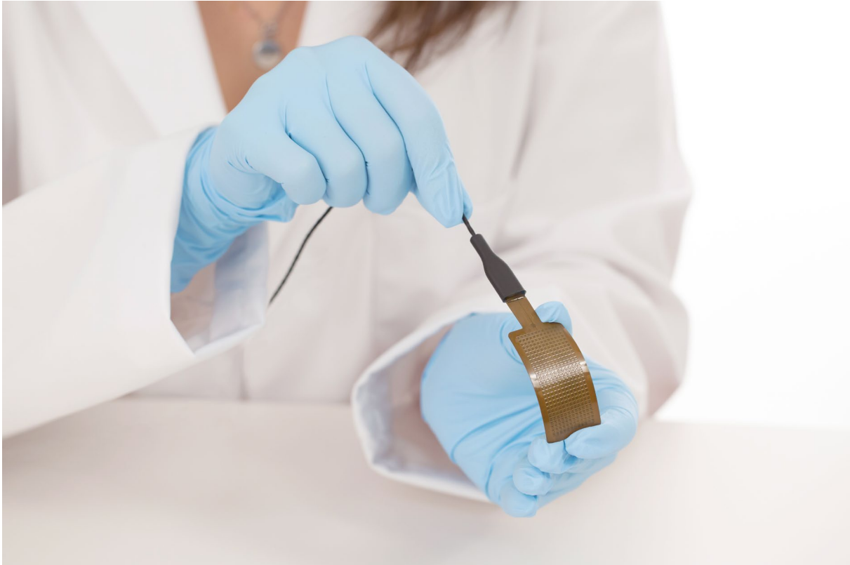
Figure 2.2 Heat flux from the back side to the front side generates a positive voltage output signal. The dot on the foil indicates the front side.
