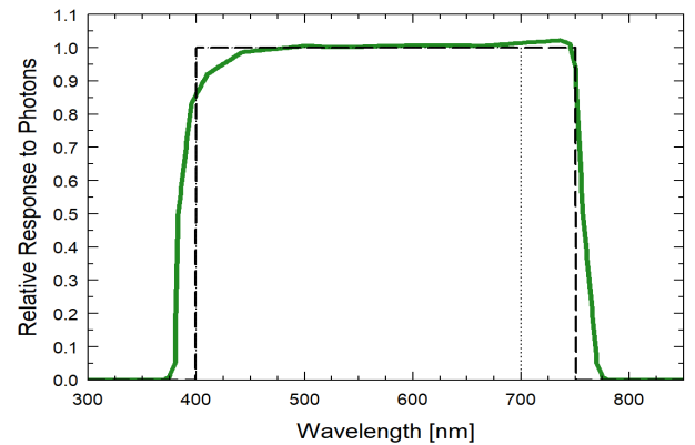
Spectral response of the ePAR sensor (green) compared to the "ePAR" target response (dashed) and the traditional PAR response (dotted).
